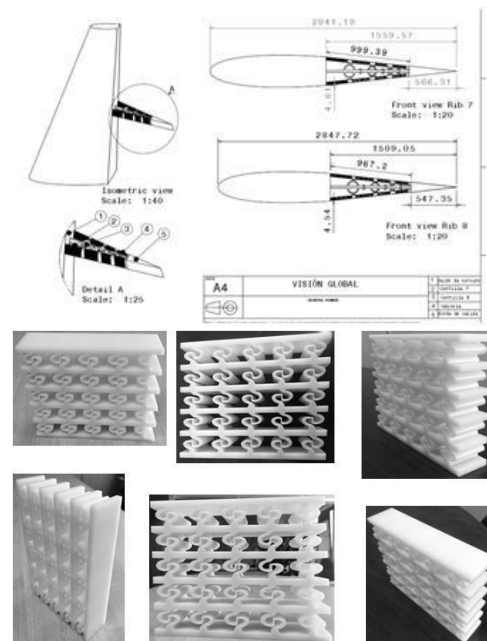
Figure 1. Morphing rudder structural architecture and 3D printed detail.
