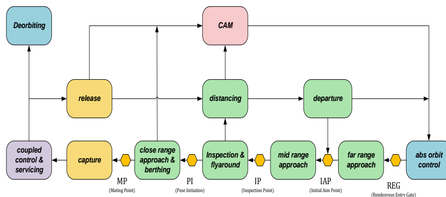
Figure 2 GNC Functions
