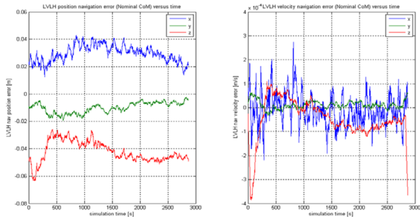
Figure 6 Simulated Lidar based navigation error during mid range approach
