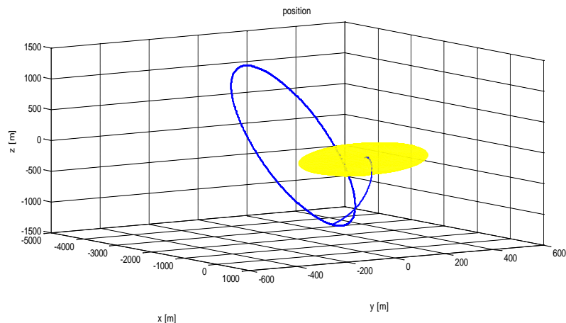
Figure 12 Typical CAM trajectory
