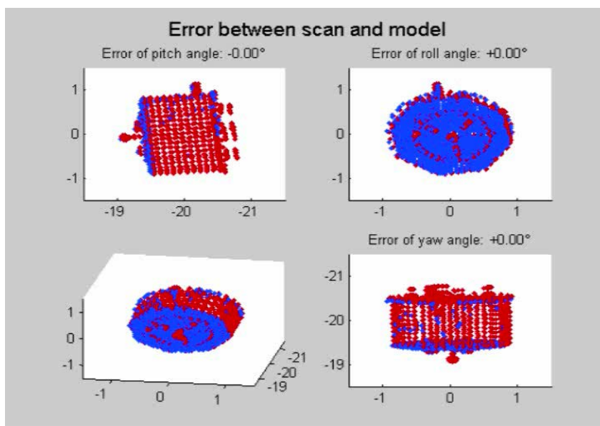
Figure 7 Simulation results of matching a model of the target satellite (red dots) with the scan data acquired by the scanning LIDAR.
