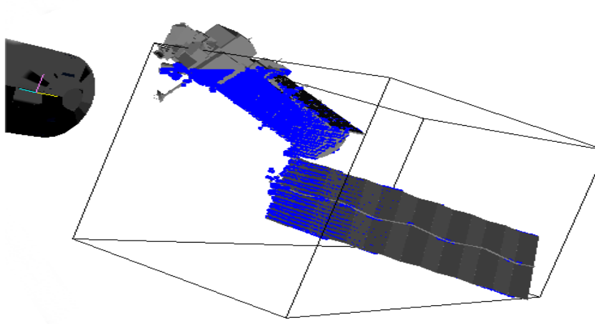
Figure 8 Simulation of a scanning LIDAR for ENVISAT as target
