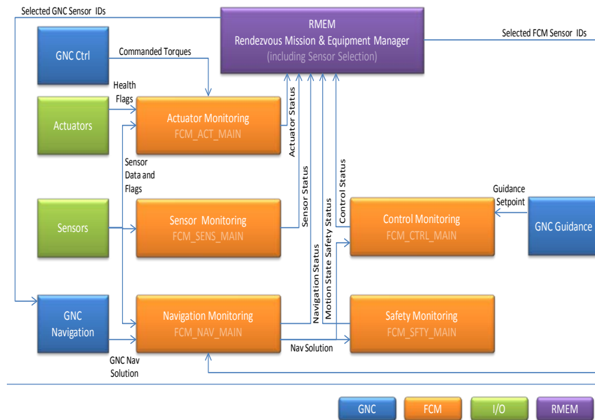
Figure 11 Flight Control Monitoring Block Diagramm
