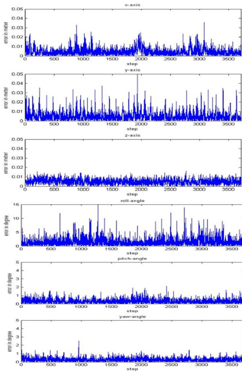
Figure 9 Simulation results for the initialization of the pose-estimation by correlation followed by the ICP algorithm over 3600 initial attitudes at a distance of 15m.
