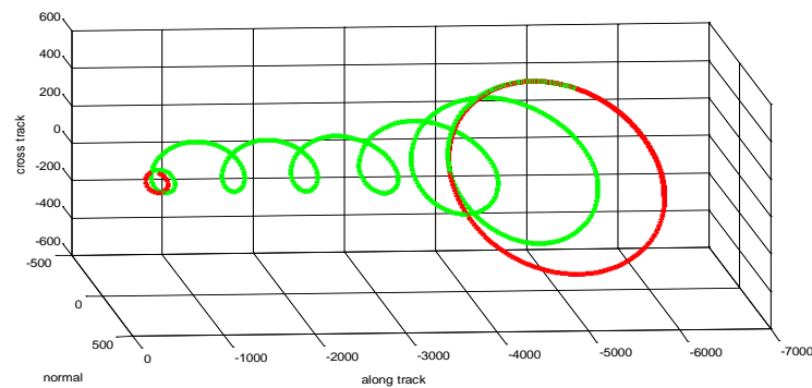
Figure 4 Formation flight and spiral approach
