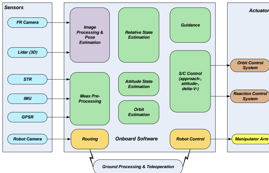
Figure 3 GNC System concept
